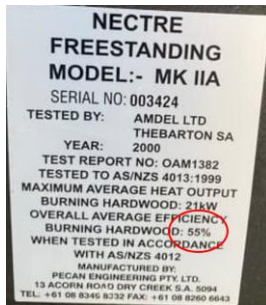
Figure 12.5 - Example slow combustion wood heater rating plate
