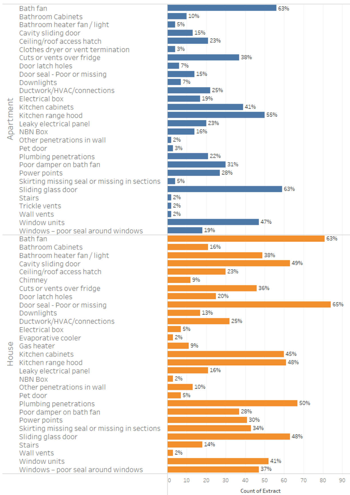
Figure 26 Identified leakage points
