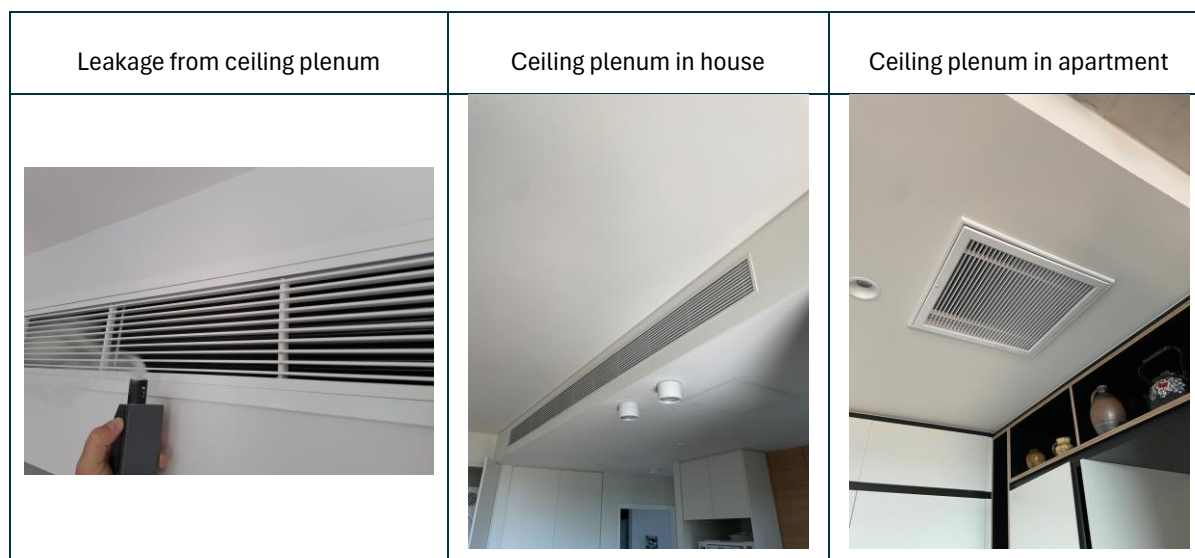
Figure 45 Ceiling plenums
