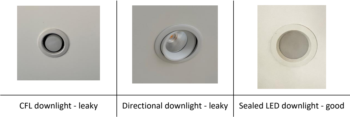
Figure 22 Downlight types
