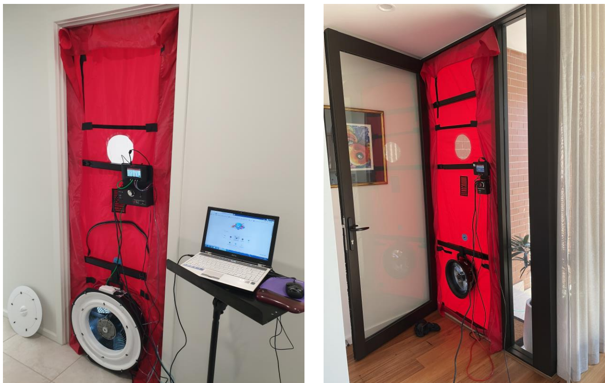
Figure 5 Typical air tightness setup
