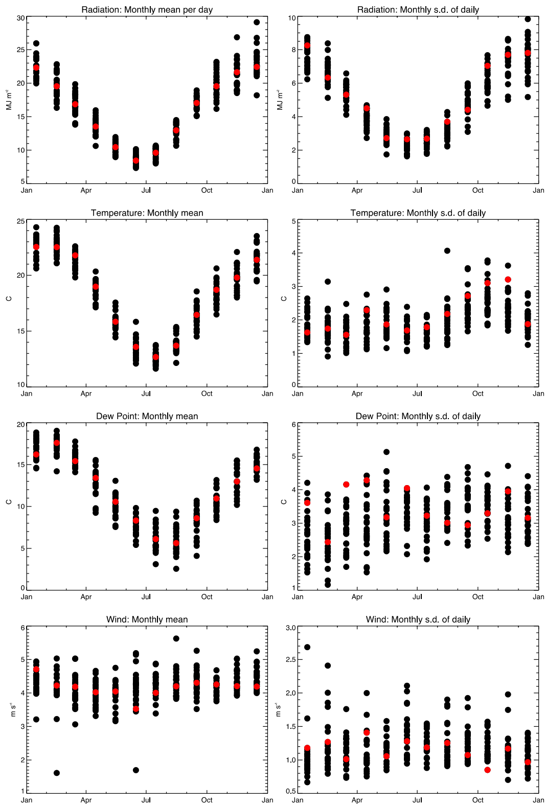
Monthly mean and standard deviation of daily climate parameters for Sydney . Red points indicate the selected months for the RMY.
