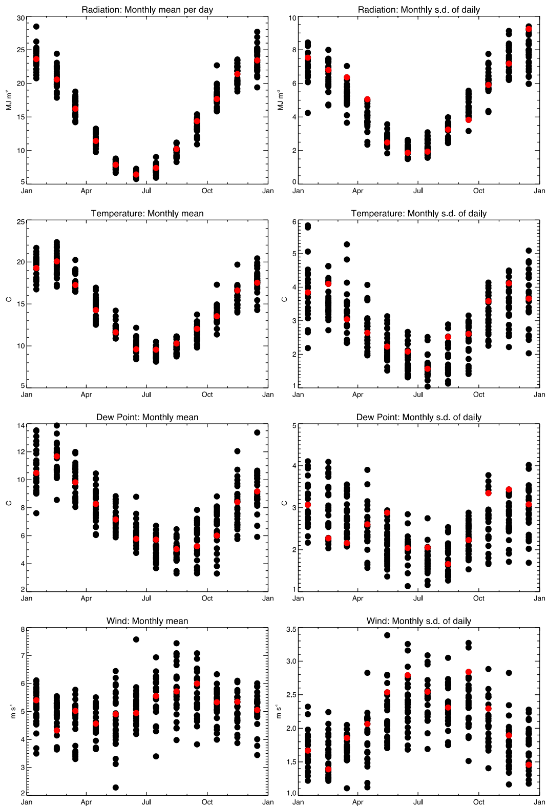
Monthly mean and standard deviation of daily climate parameters for Tullamarine . Red points indicate the selected months for the RMY.
