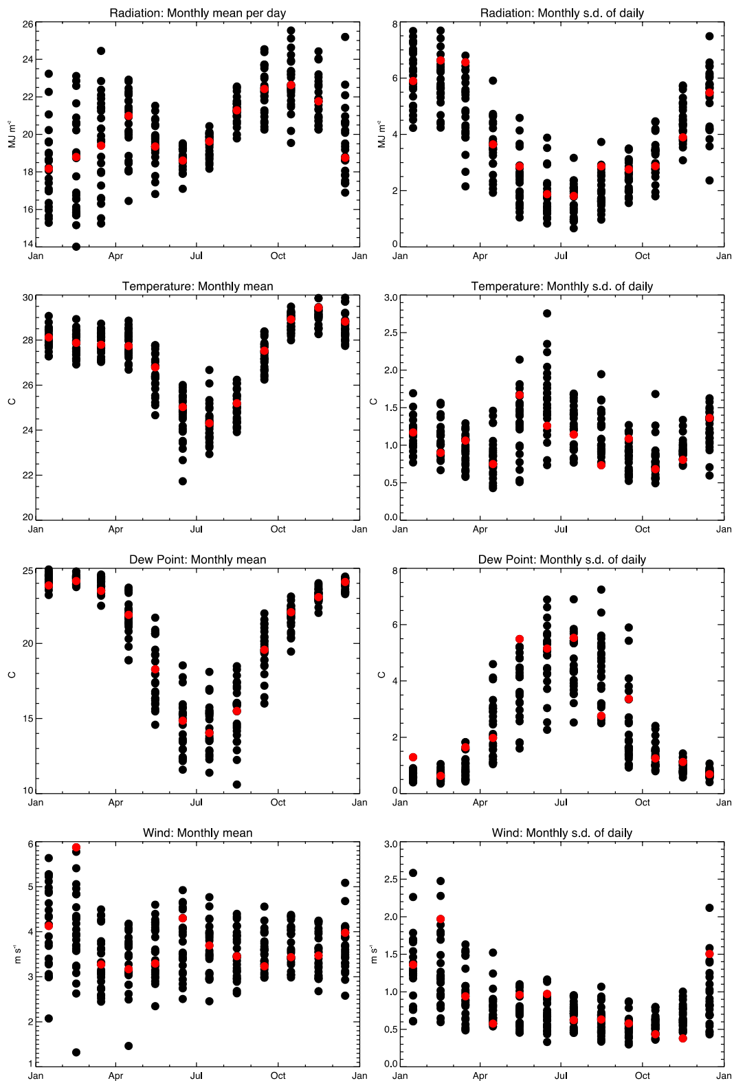
Monthly mean and standard deviation of daily climate parameters for Darwin . Red points indicate the selected months for the RMY.
