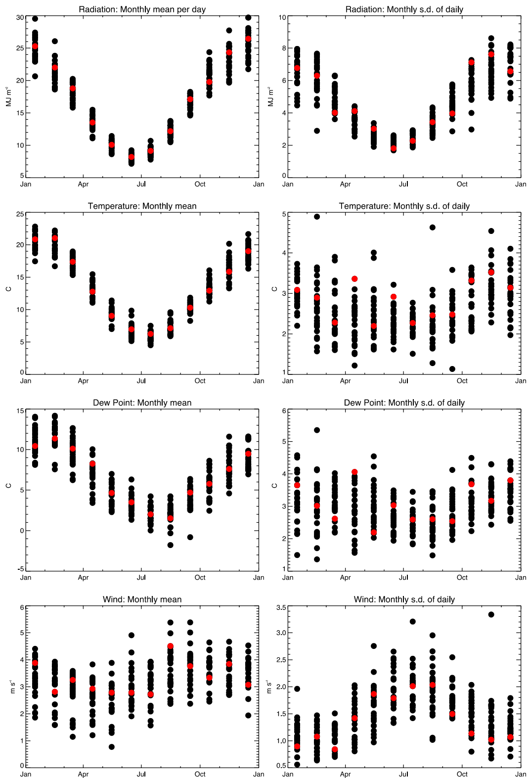
Monthly mean and standard deviation of daily climate parameters for Canberra . Red points indicate the selected months for the RMY.
