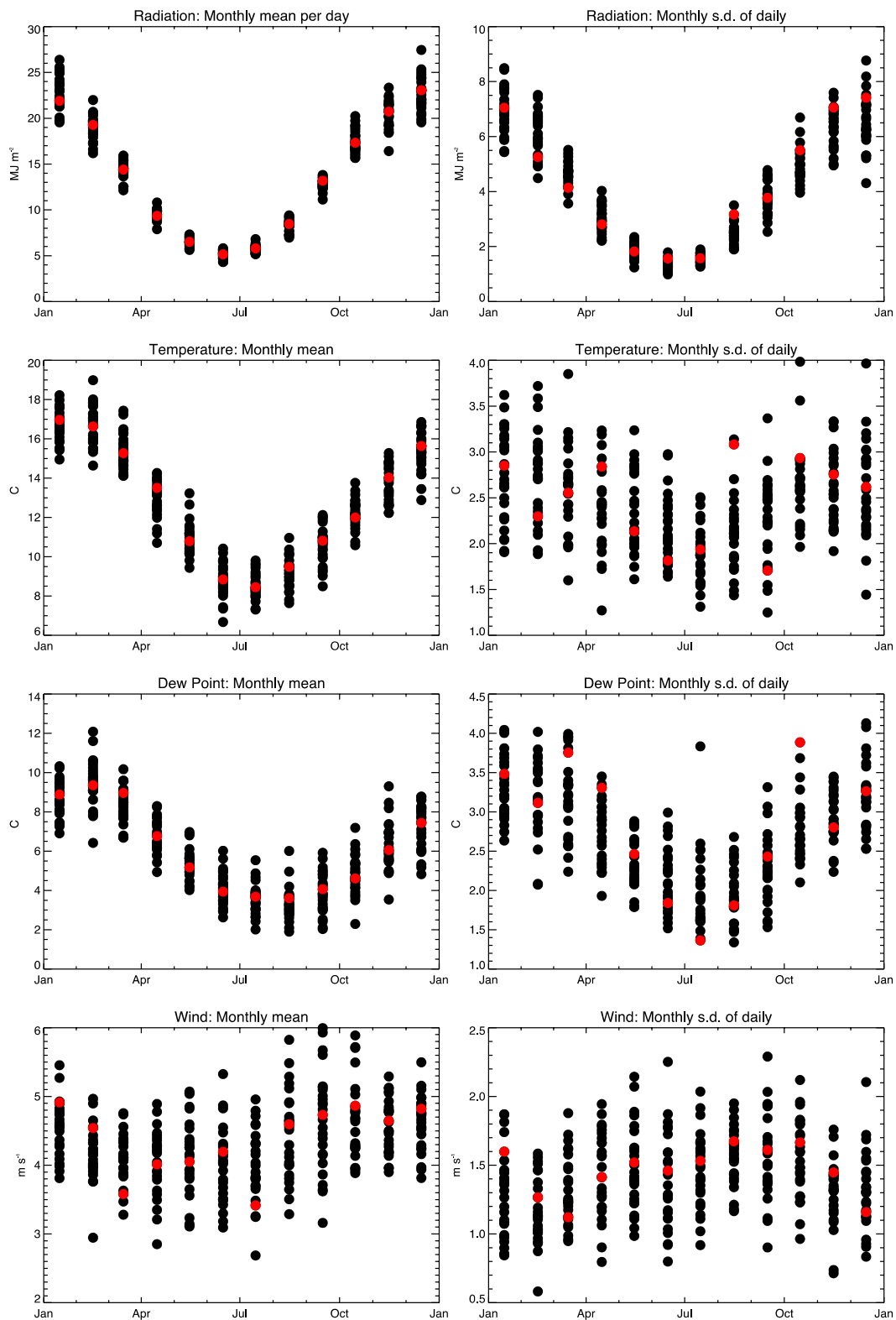
Monthly mean and standard deviation of daily climate parameters for Hobart . Red points indicate the selected months for the RMY.
