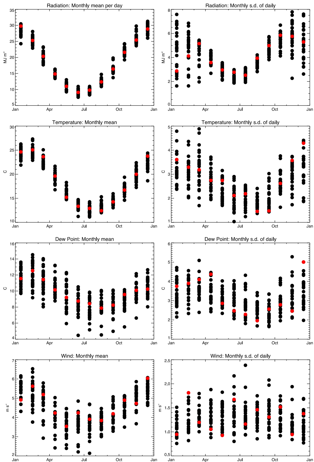
Monthly mean and standard deviation of daily climate parameters for Perth . Red points indicate the selected months for the RMY.
