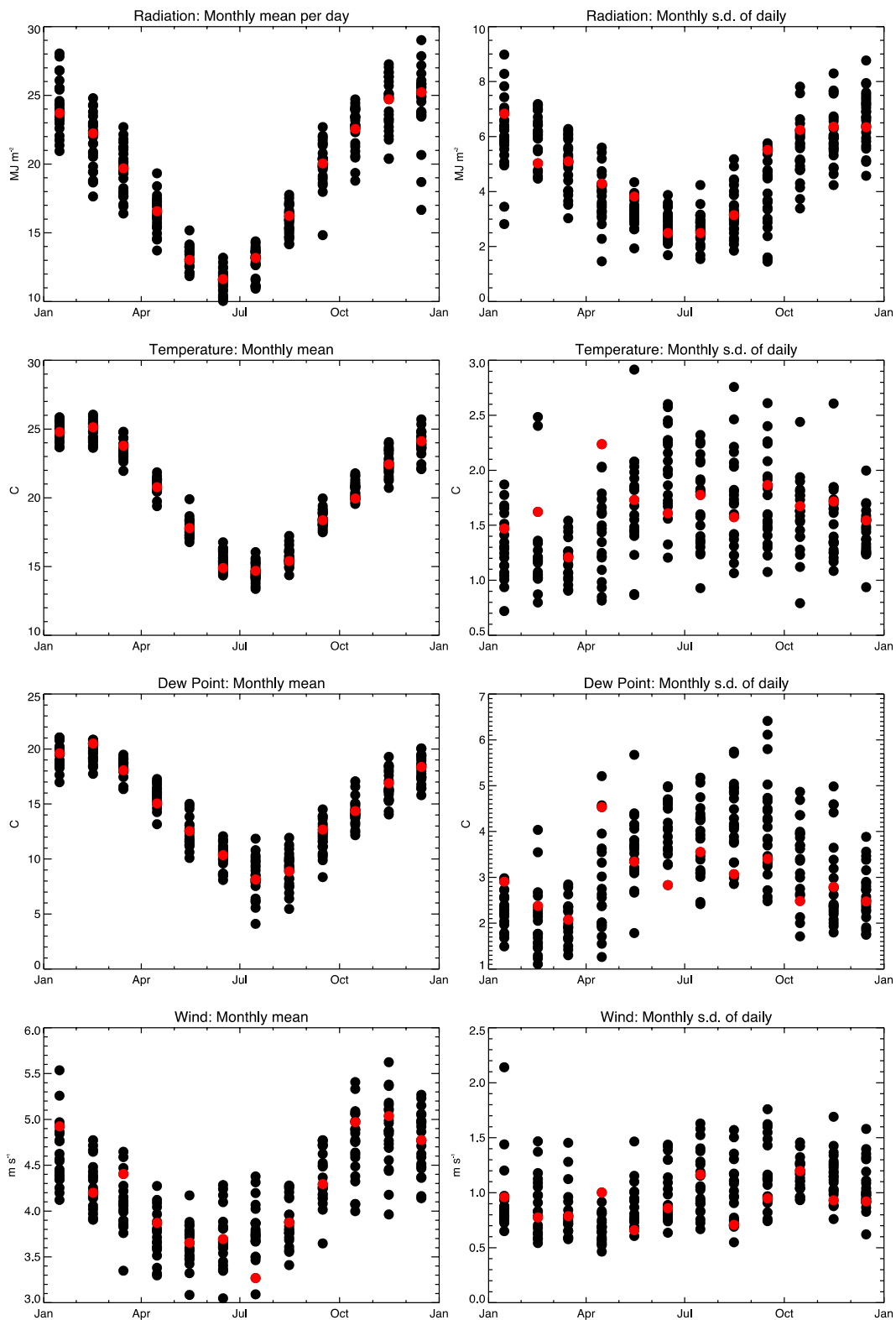
Monthly mean and standard deviation of daily climate parameters for Brisbane . Red points indicate the selected months for the RMY.
